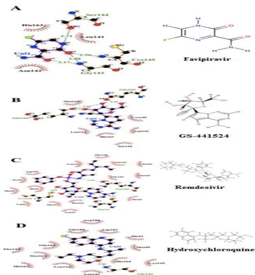
Figure 4. The inhibitory binding interactions of A) Favipiravir; B) GS-441524; C) Remdesivir; D) Hydroxychloroquine with the active amino acids of the SARS-CoV-2 Mpro (hydrogen bonds are represented in green-dotted lines).
