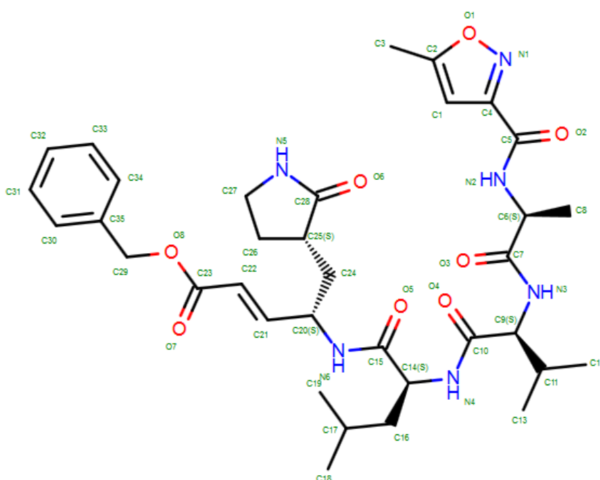
Figure. 1. Chemical Structure (numbered) of the inhibitor N3 of SARS-CoV-2 Mpro ( IUPAC Nomenclature : N -[(5-Methylisoxazol-3-yl)carbonyl]alanyl-L-valyl- N -1-~((1 R ,2 Z )-4-(benzyloxy)-4-oxo-1-~{(3 R )-2-oxopyrrolidin-3-yl)methyl}but-2-enyl)-L-leucinamide).
