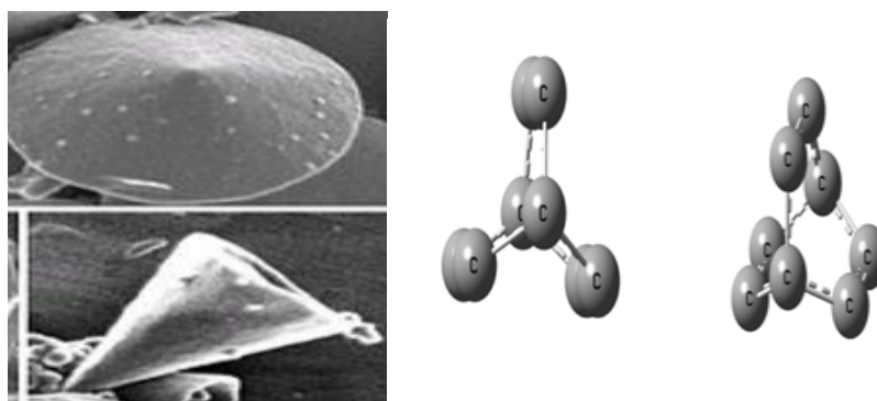
Fig1: Carbon nano cone from three view
