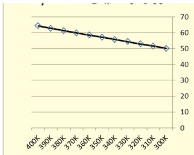
Fig (4) diagram of \Delta G_f amounts of Boric acid desolation process in water result in B(OH)_4^- and hydronium ion.
