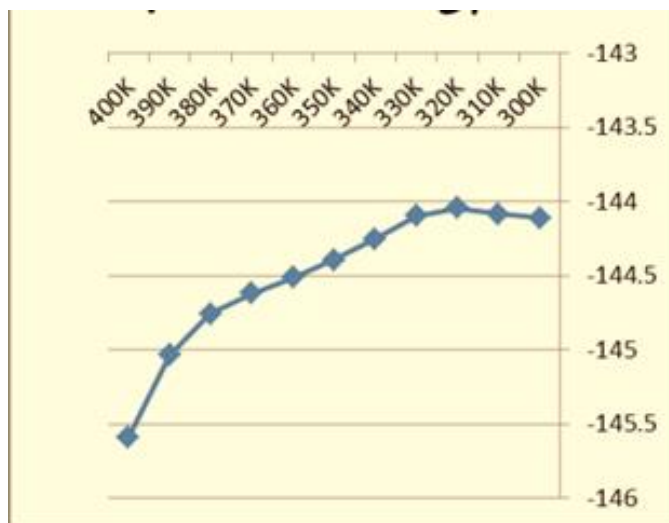
Fig (2) the diagram of entropy changes of boric acid desolation process in water result in B(OH)_4^- and hydronium ion.
