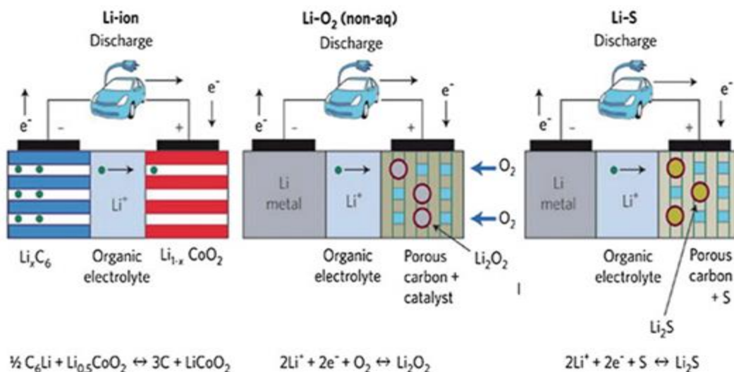
Figure 4. Schematic representation of Li-ion, non-aqueous Li–O 2 , and Li–S batteries. [29] Copyright 2016 Royal Society of Chemistry.
