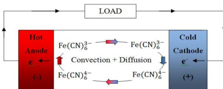
Figure 5. Ferro-/ferricyanide redox thermogalvanic cell [36] Copyright by 2012 Springer.
