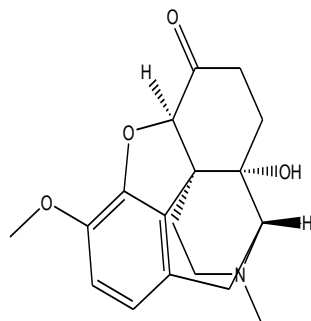
(5R,9R,13S,14S)-4,5a-Epoxy-14-hydroxy-3-methoxy-17-methylmorphinan-6-one
